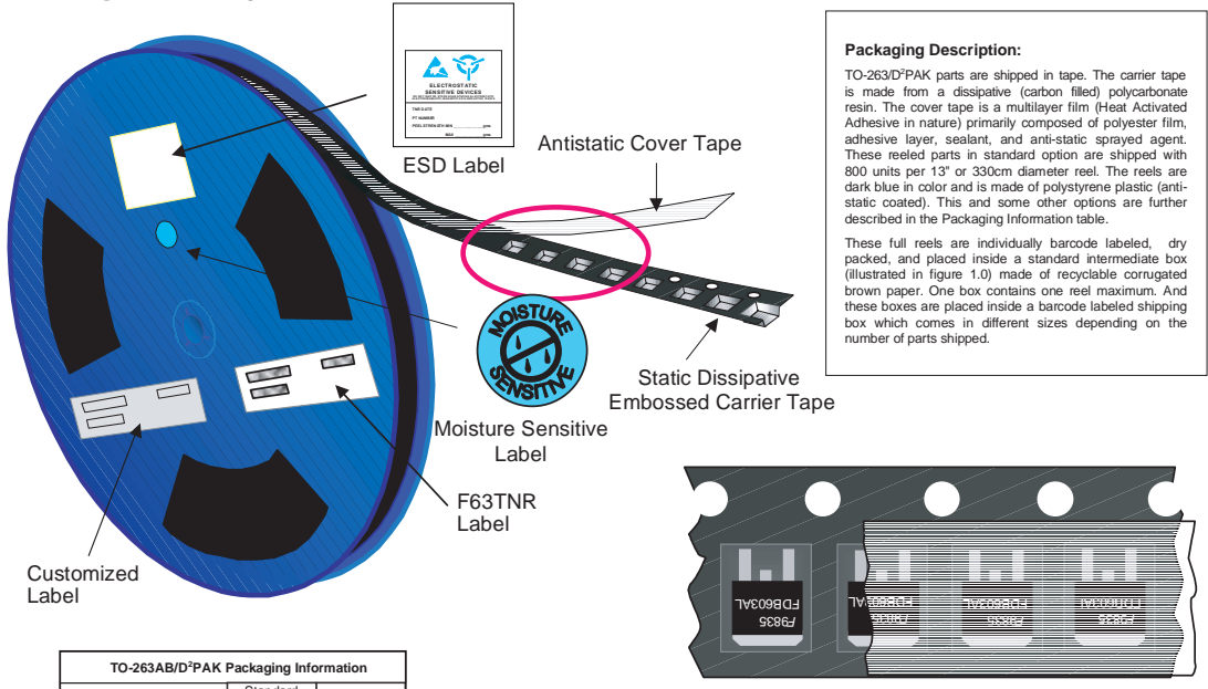
TO-263AB/D 2 PAK Packaging Configuration: Figure 1.0
